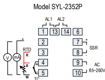
Figure 1. Wiring terminals of SYL-2352P.
