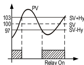
Figure 5. On/off control mode.
